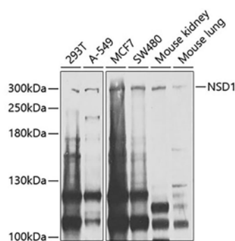
Fig. 1. Western blot analysis of extracts of various cell lines, using NSD1 antibody at 1:1000 dilution. Secondary antibody: HRP-labeled Goat Anti-Rabbit IgG(H+L) (A0208) at 1:1000 dilution. Lysates/proteins: 25 \mu g per lane. Blocking buffer: QuickBlock™ Blocking Buffer (P0231). Detection: BeyoECL Star (P0018A). Exposure time:1s.
